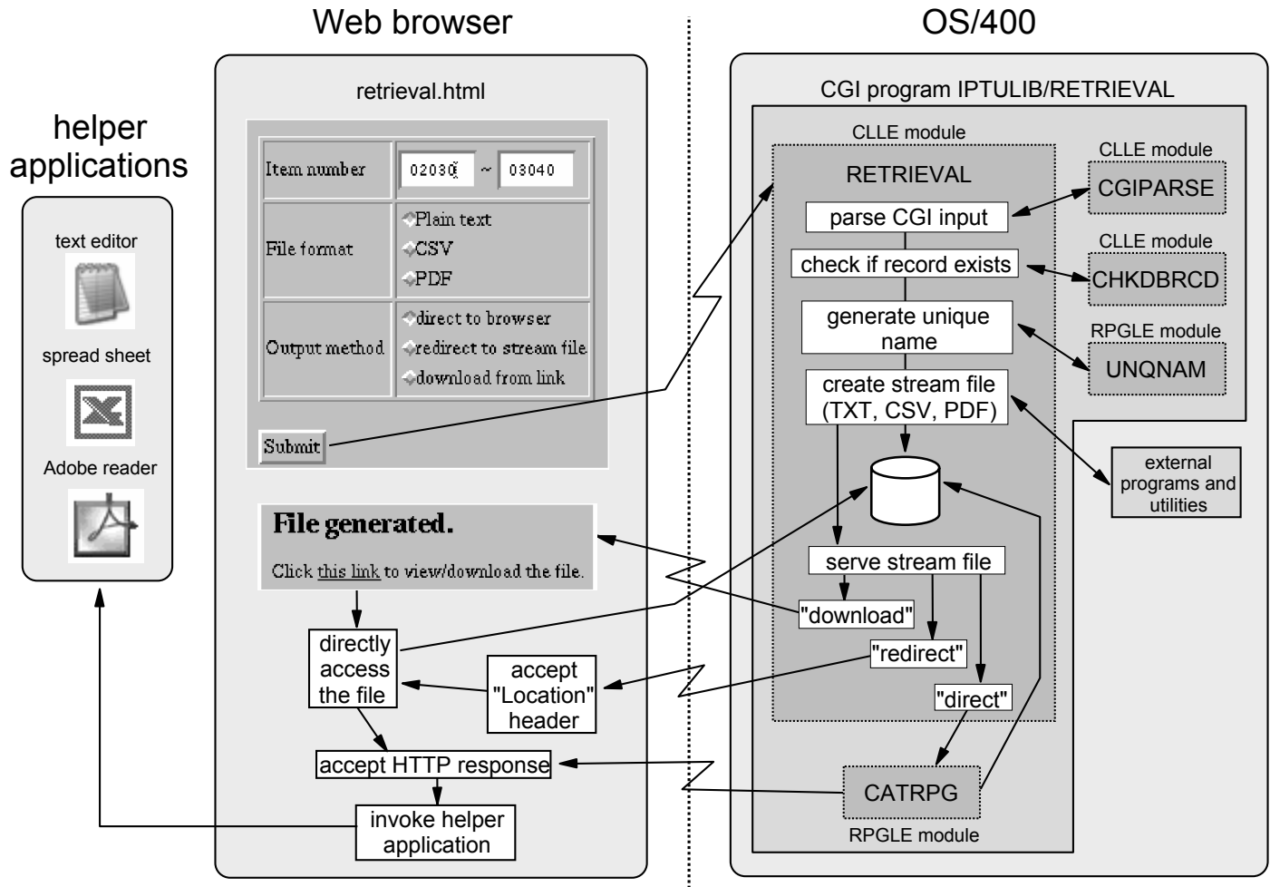
Figure 133 – A Direct File Retrieval Application
